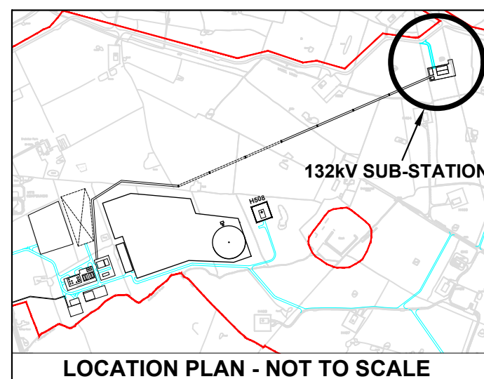
FIGURE 2.12 - HOLFORD BRINEFIELD - KGSP - 132kV SUB-STATION - CONSENTED DEVELOPMENT LIMITS OF DEVIATION VS PROPOSED DEVELOPMENT LIMITS OF DEVIATION - ABOVE GROUND
